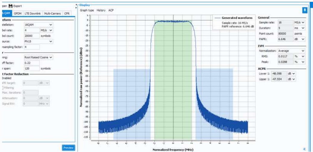
WAVEFORM GENERATOR
