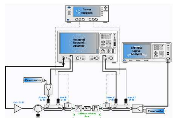
Vector Setup for 1-Tone and S-Par Measurements (IQS100B-10 and B-11)
